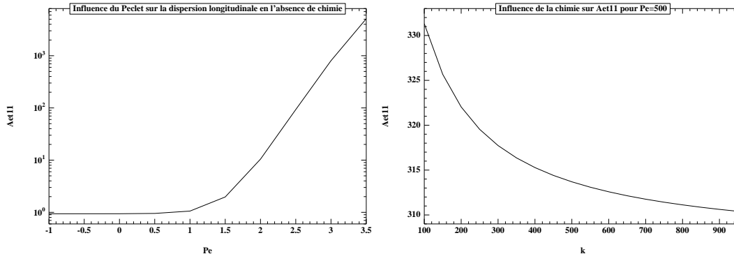
Figure 1. Log-log plot of A_{11}^* in terms of the Péclet number with k = 0 (left). Variation of A_{11}^* in terms of the Damkohler number k with a fixed Péclet number (right).
